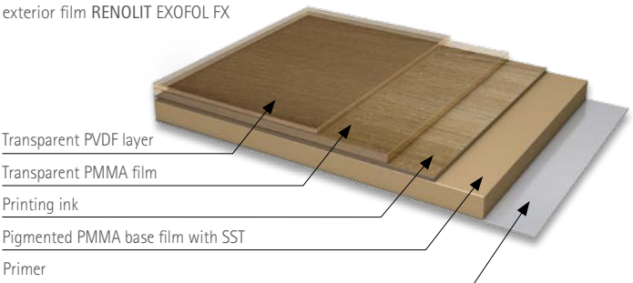
Diagram showing the structure of the exterior film RENOLIT EXOFOL FX
